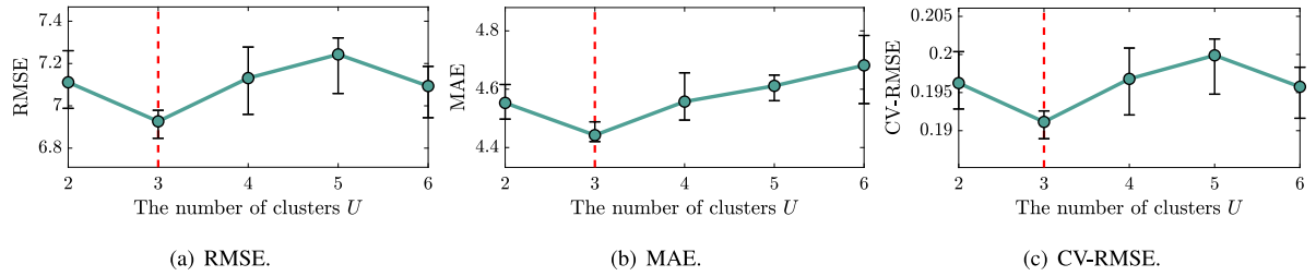
Fig. 8. The GAIN performance with varying the number of clusters U in terms of three metrics.
