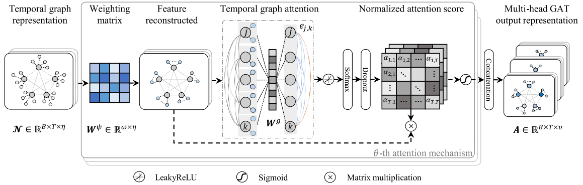
Fig. 6. The multi-head graph attention architecture in the proposed GAIN.
