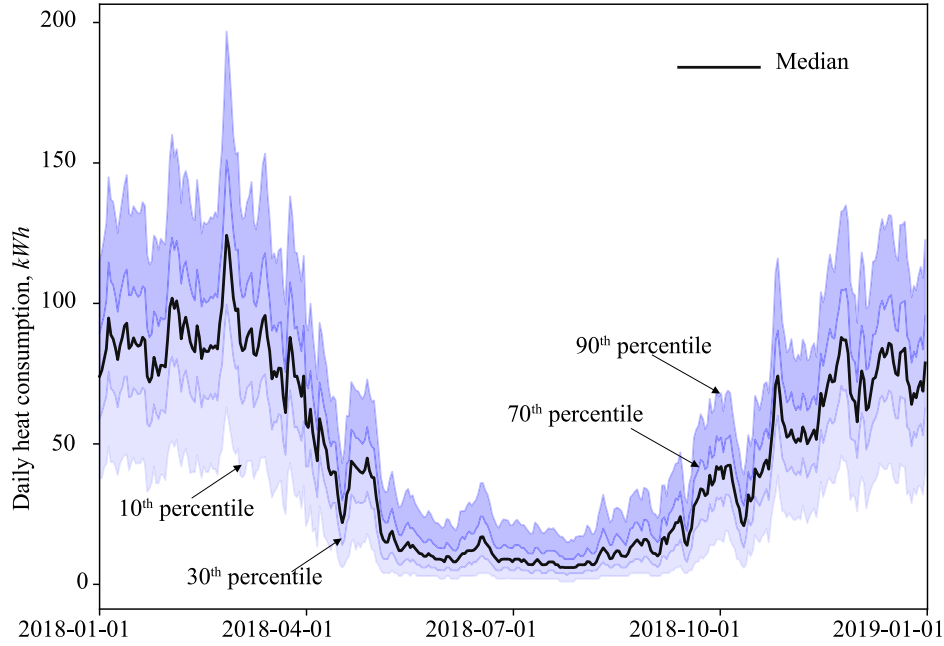
Fig. 4. Percentiles of heat load.
