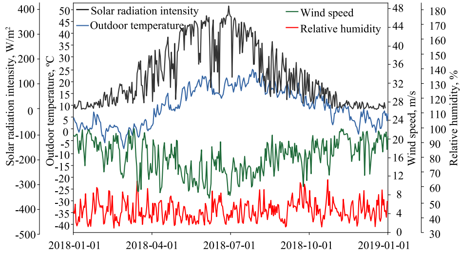
Fig. 3. Outdoor meteorological parameters.
