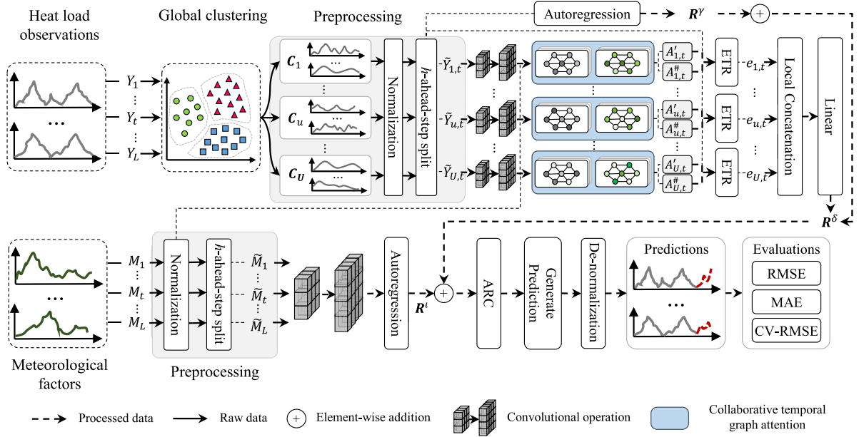
Fig. 5. Overview of the proposed GAIN model.
