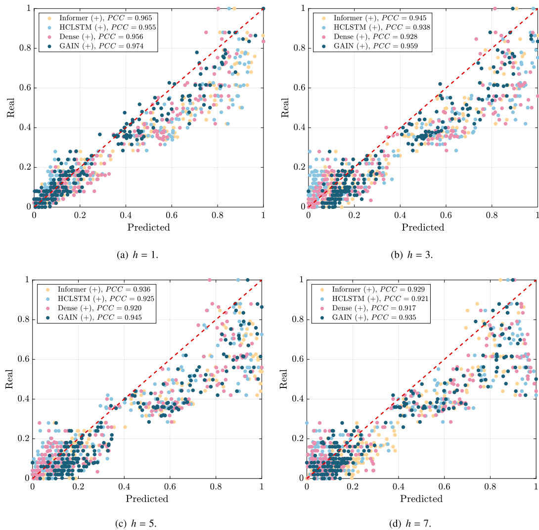
Fig. 13. The correlation visualizations of GAIN(+) predictions and four other benchmark predictions; Unit of h : day.
