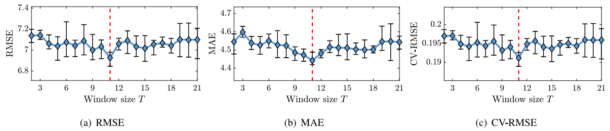
Fig. 7. The GAIN performance by varying the window size T in terms of three metrics. For each metric, the optimal value is found at red dash line.
