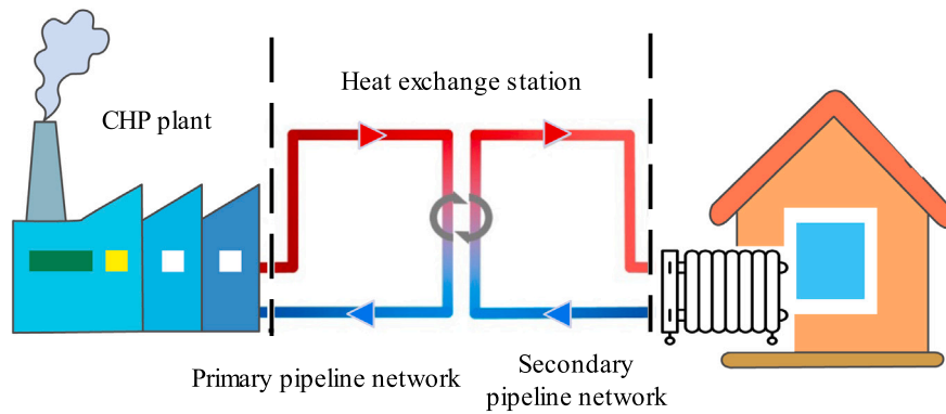
Fig. 1. Schematic diagram of district heating system.
