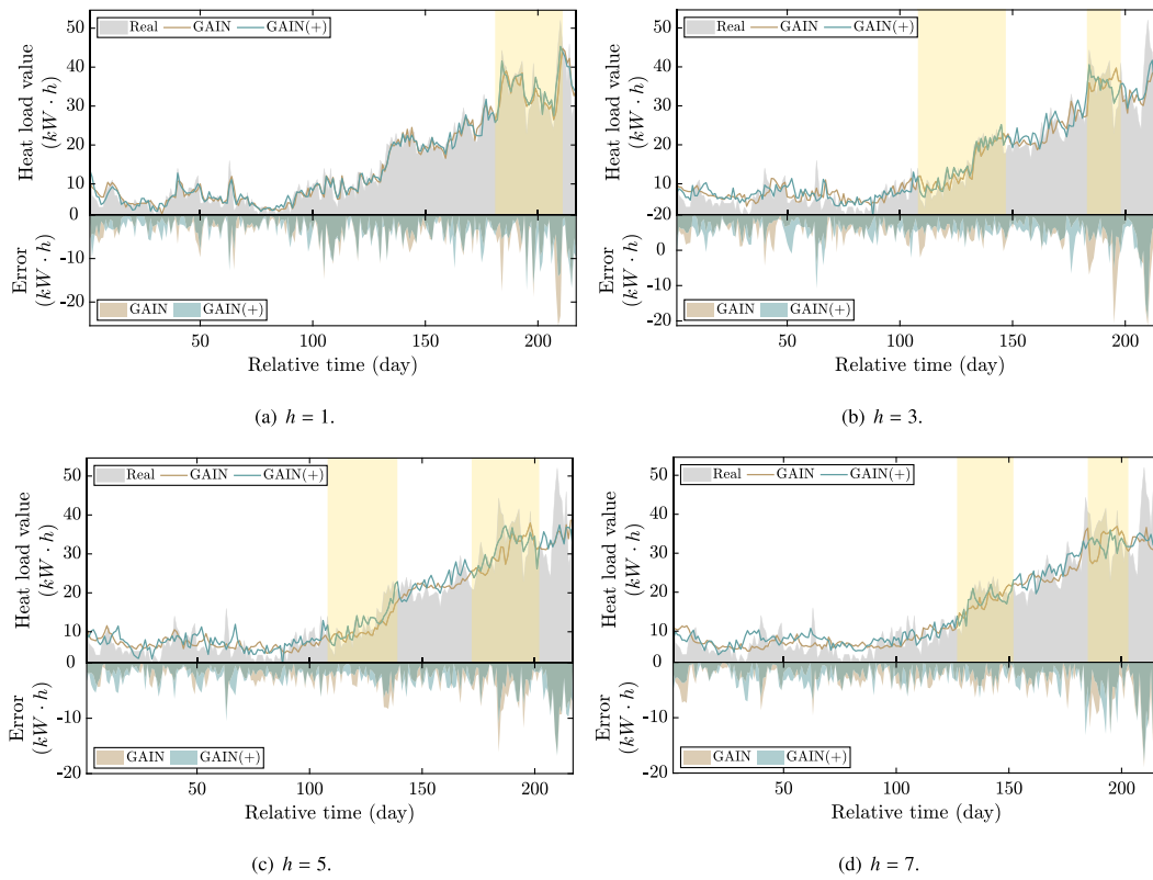
Fig. 9. The visualizations among real values, GAIN predictions, and GAIN(+) predictions and prediction error; Unit of h : day.
