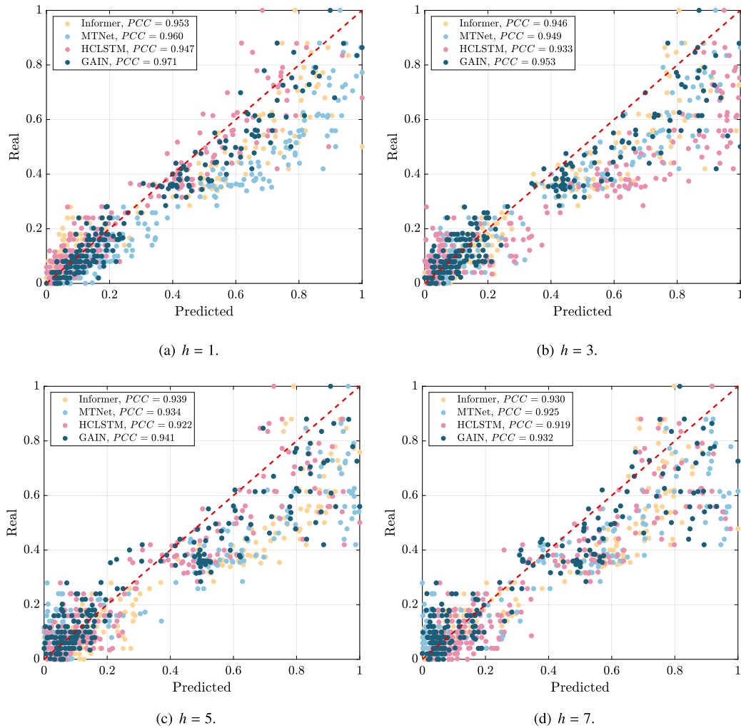
Fig. 11. The correlation visualizations of GAIN predictions and four other benchmark predictions; Unit of h : day.
